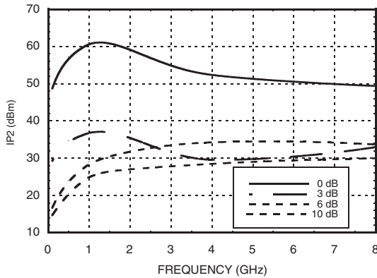
Input Second Order Intercept vs. Attenuation*
