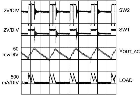
Typical Switching Waveform in Boost Mode (PFM Mode)
