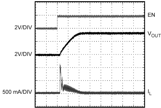
Start up in PWM Mode ( V_{OUT} = 3.4V, Load = 1mA )
