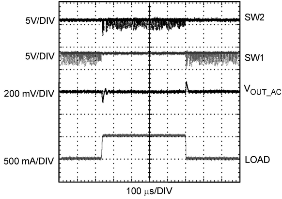
Load Transient in Buck-Boost Operation (Forced PWM Mode) V_{IN} = 3.44V, V_{OUT} = 3.4V, \text{Load} = 0-500mA
