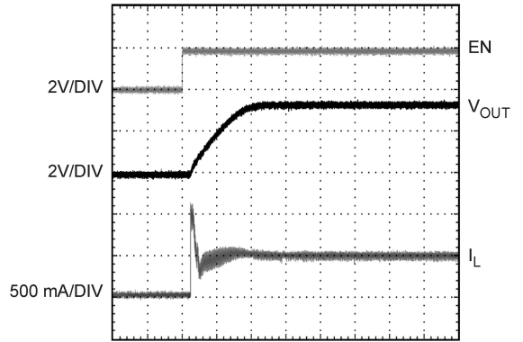
Start up in PWM Mode ( V_{OUT} = 3.4V, Load = 500mA )
