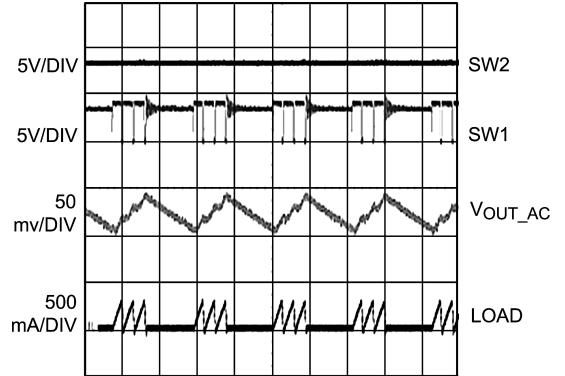
Typical Switching Waveform in Buck Mode (PFM Mode)
