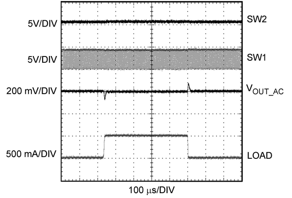
Load Transient in Buck Mode (Forced PWM Mode) V_{IN} = 4.2V, V_{OUT} = 3.0V, \text{Load} = 0-500mA
