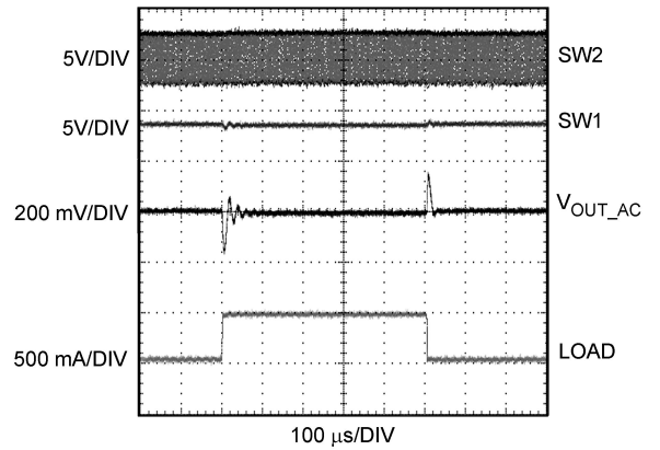
Load Transient in Boost Mode (Forced PWM Mode) V_{IN} = 3.5V, V_{OUT} = 5.0V, \text{Load} = 0-500mA
