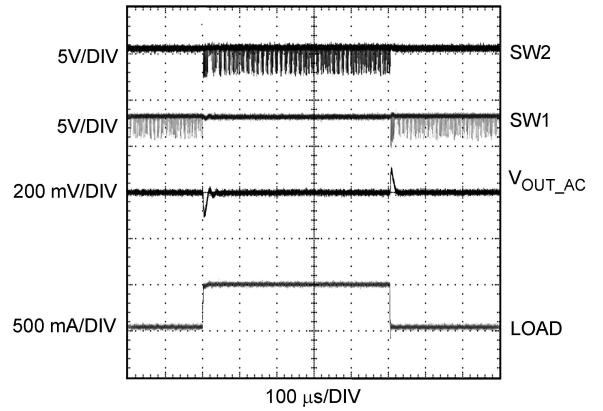
Load Transient in Buck-Boost Mode (Forced PWM Mode) V_{IN} = 3.05V, V_{OUT} = 3.0V, \text{Load} = 0-500mA
