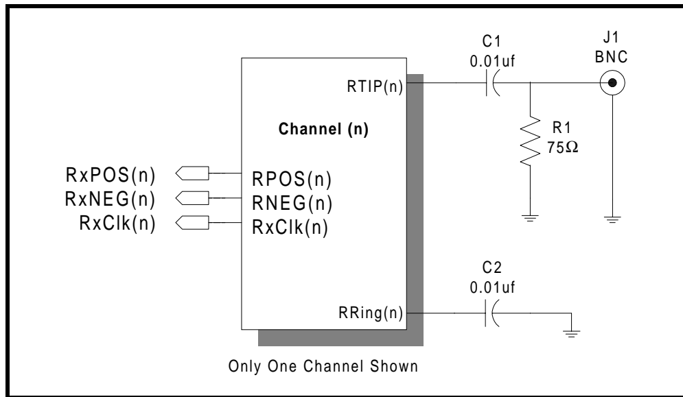
FIGURE 16. RECOMMENDED SCHEMATIC FOR CAPACITIVE-COUPLING THE RECEIVE SECTION OF THE XRT7302 TO THE LINE
