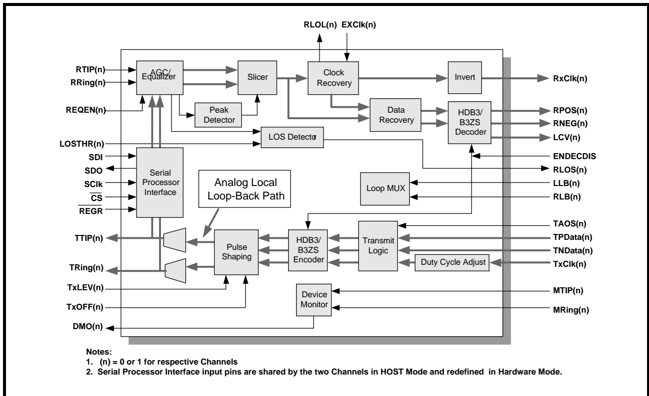
FIGURE 27. A CHANNEL IN THE XRT7302 OPERATING IN THE ANALOG LOCAL LOOP-BACK MODE
