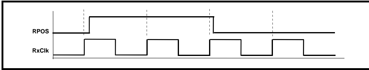
FIGURE 26. THE BEHAVIOR OF THE RPOS AND RxClk OUTPUT SIGNALS WHILE THE XRT7302 IS TRANSMITTING SINGLE-RAIL DATA TO THE RECEIVING TERMINAL EQUIPMENT
