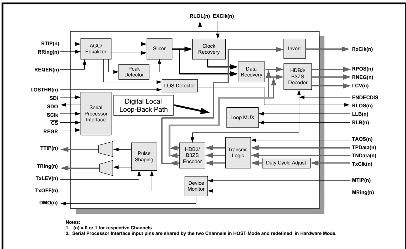
FIGURE 28. THE DIGITAL LOCAL LOOP-BACK PATH IN A GIVEN CHANNEL OF THE XRT7302
