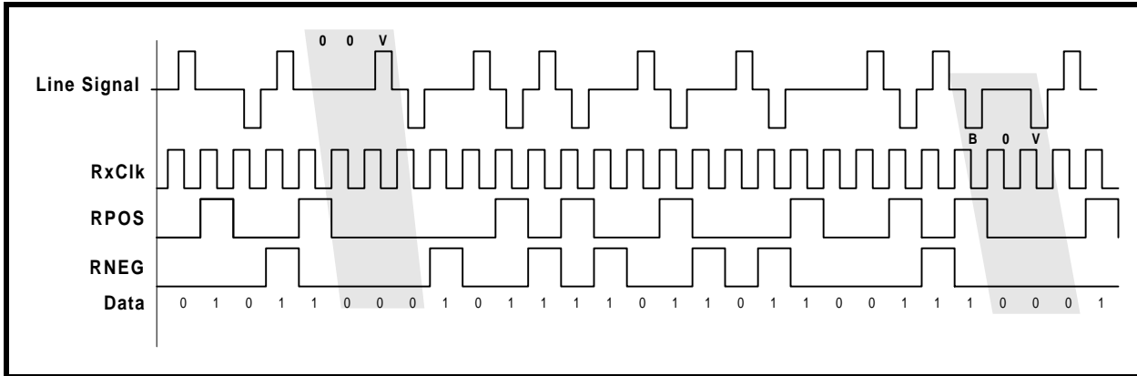
FIGURE 18. AN EXAMPLE OF B3ZS DECODING
