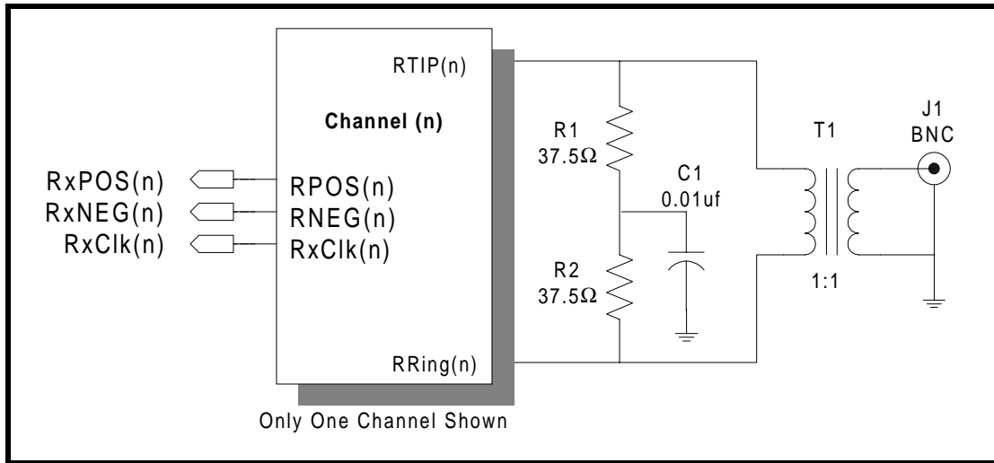
FIGURE 15. RECOMMENDED SCHEMATIC FOR TRANSFORMER-COUPLING THE RECEIVE SECTION OF THE XRT7302 TO THE LINE
