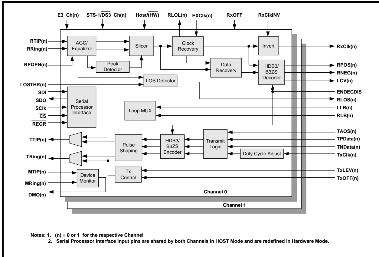
FIGURE 6. FUNCTIONAL BLOCK DIAGRAM OF THE XRT7302
