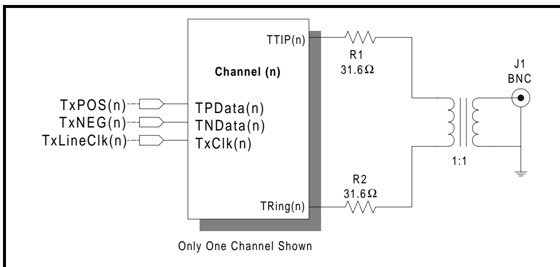
FIGURE 14. RECOMMENDED SCHEMATIC FOR INTERFACING THE TRANSMIT SECTION OF THE XRT7302 TO THE LINE
