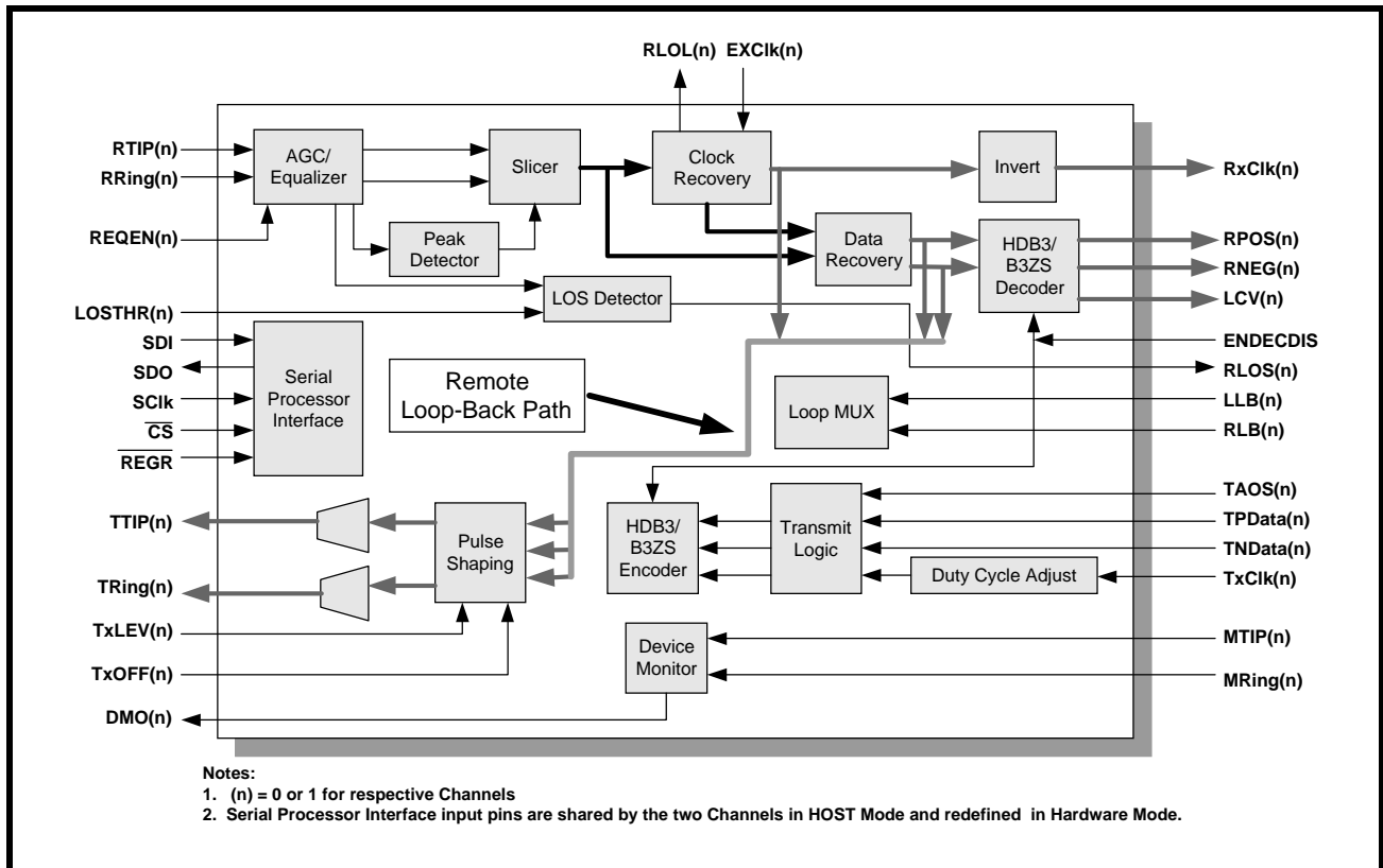
FIGURE 29. THE REMOTE LOOP-BACK PATH IN A GIVEN XRT7302 CHANNEL
