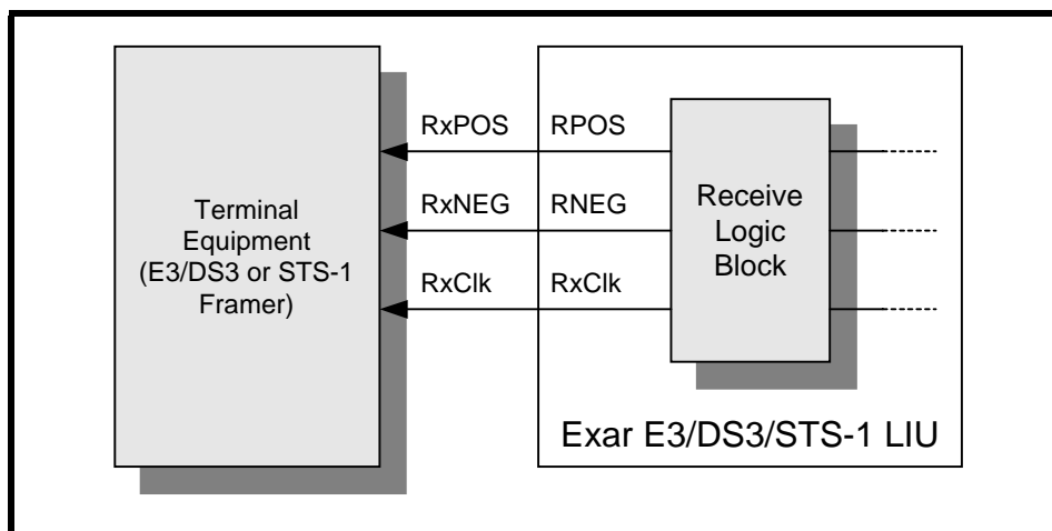
FIGURE 22. THE TYPICAL INTERFACE FOR THE TRANSMISSION OF DATA IN A DUAL-RAIL FORMAT FROM THE RECEIVE SECTION OF THE XRT7302 TO THE RECEIVING TERMINAL EQUIPMENT
