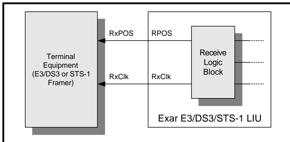
FIGURE 25. THE TYPICAL INTERFACE FOR DATA TRANSMISSION IN A SINGLE-RAIL FORMAT FROM THE RECEIVE SECTION OF THE XRT7302 TO THE RECEIVING TERMINAL EQUIPMENT
