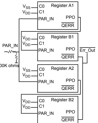
Signals for Address and Command Parity Function (M393T5750CZA)
