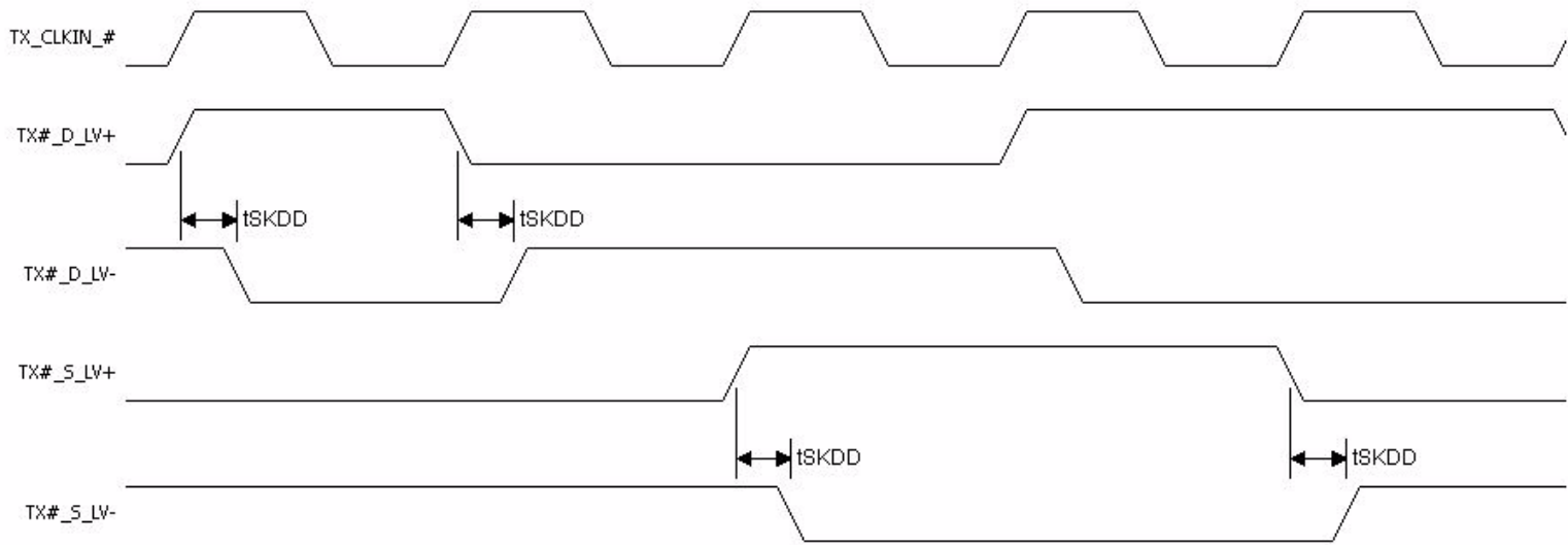
Figure 21. LVDS Driver tSKDD Timing Diagram
