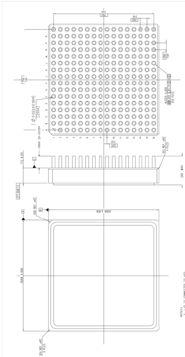
Figure 38. 255-CCGA
