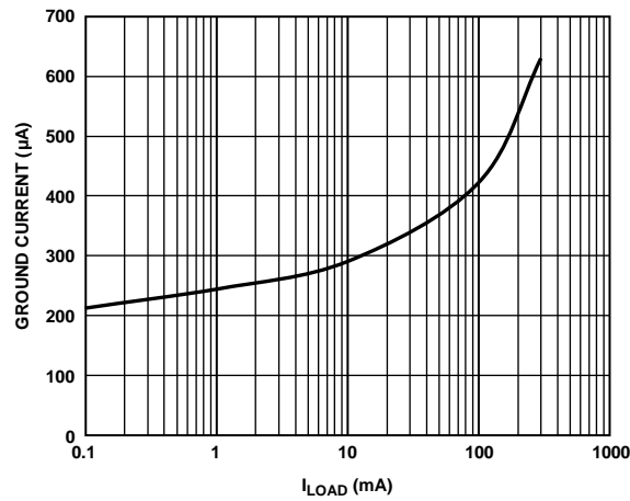
Figure 28. Ground Current vs. Load Current, V_{OUT} = 1.8V
