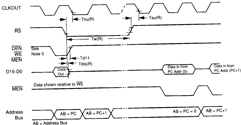
FIGURE 4 - RESET TIMING
