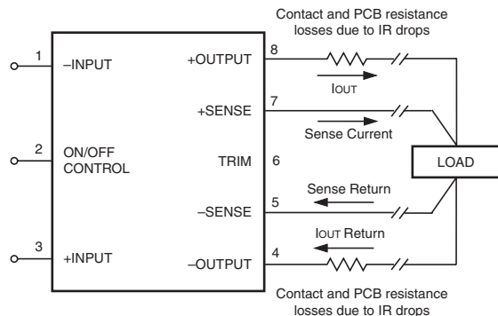
Figure 15. Remote Sense Circuit Configuration
