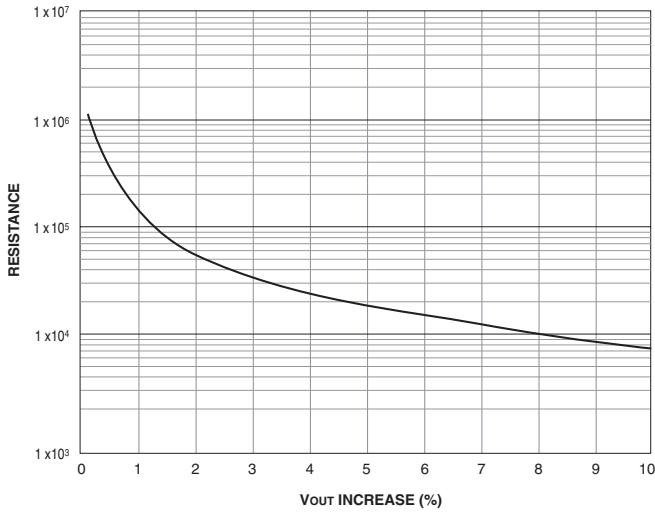
Figure 9. USQ-1.5 Trim-Up Resistance vs. % Increase Vout
