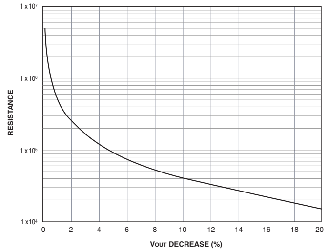
Figure 14. USQ-1.5 to USQ-3.3 Trim-Down Resistance vs. % Decrease Vout
