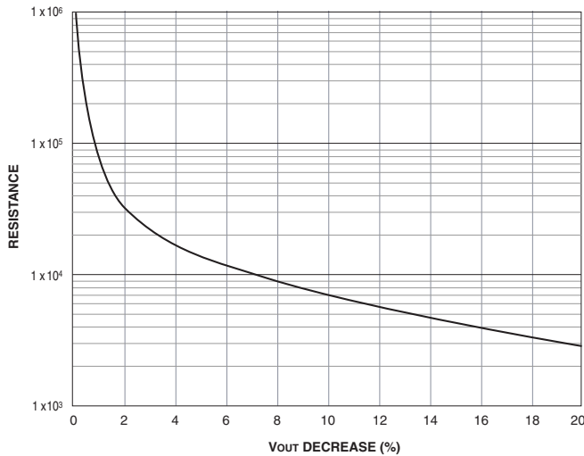
Figure 13. USQ-1.2 Trim-Down Resistance vs. % Decrease Vout
