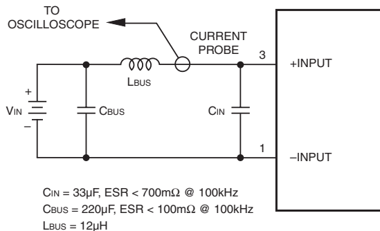
Figure 2. Measuring Input Ripple Current
