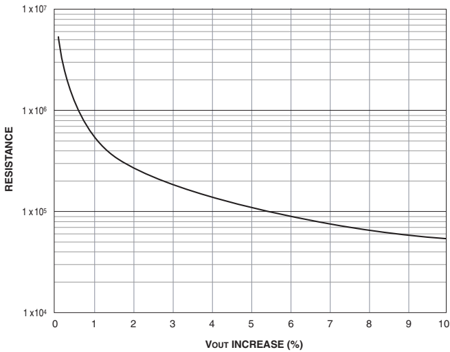
Figure 11. USQ-2.5 Trim-Up Resistance vs. % Increase Vout
