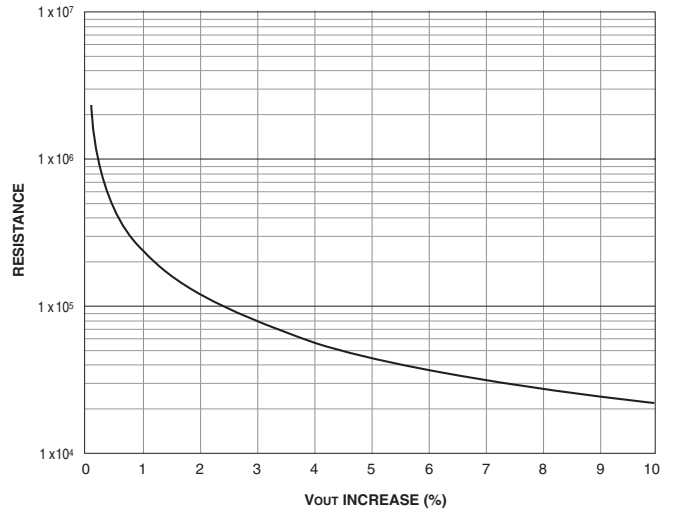
Figure 10. USQ-1.8 Trim-Up Resistance vs. % Increase Vout
