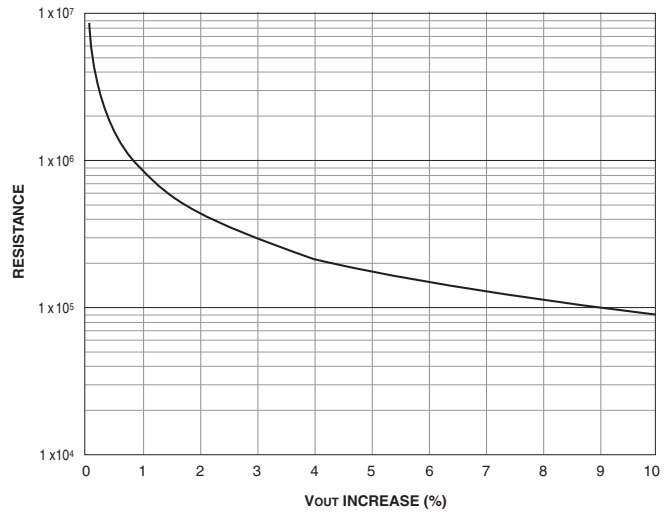
Figure 12. USQ-3.3 Trim-Up Resistance vs. % Increase Vout
