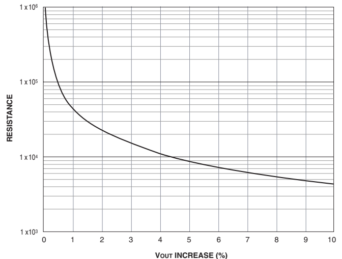
Figure 8. USQ-1.2 Trim-Up Resistance vs. % Increase Vout
