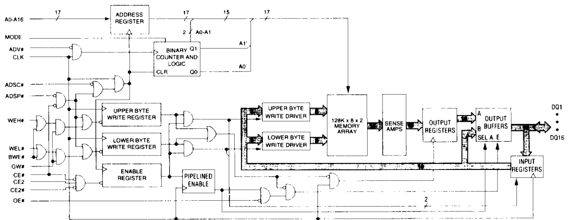
FUNCTIONAL BLOCK DIAGRAM 128K x 16
