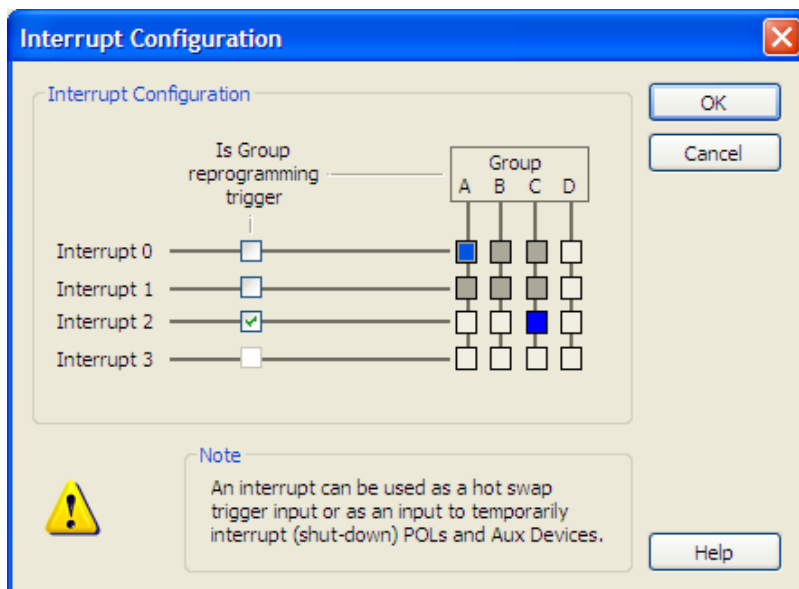
Figure 18. Interrupt Configuration Window
