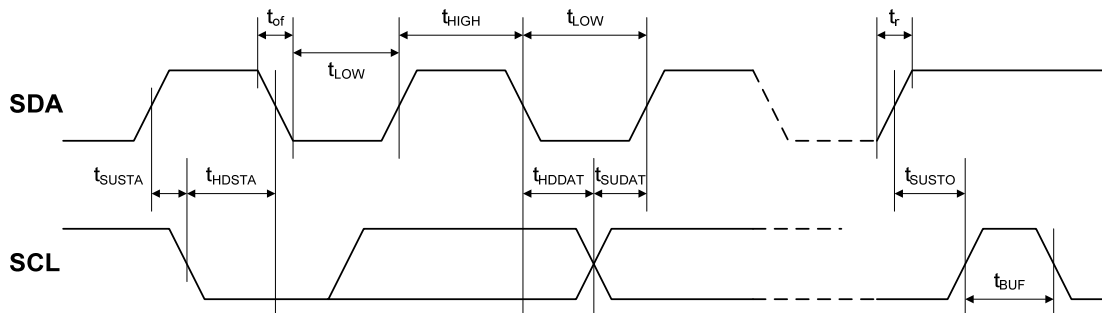
Figure 2. I 2 C Timing Parameters
