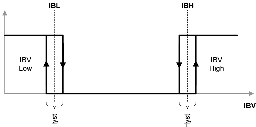
Figure 13: Undervoltage (IBL) and Overvoltage (IBH) Protections Hysteresis
