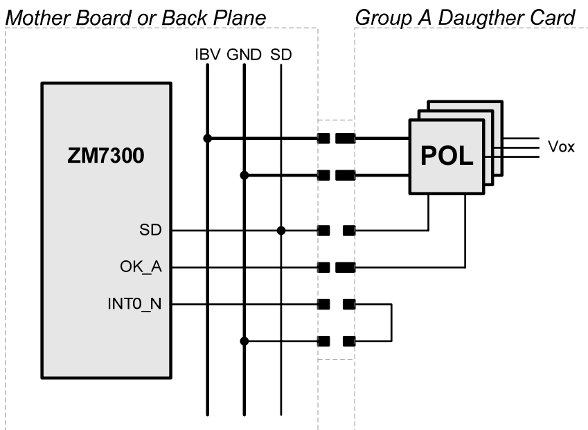
Figure 19: INT0 Configured as Group A Reprogramming Trigger
