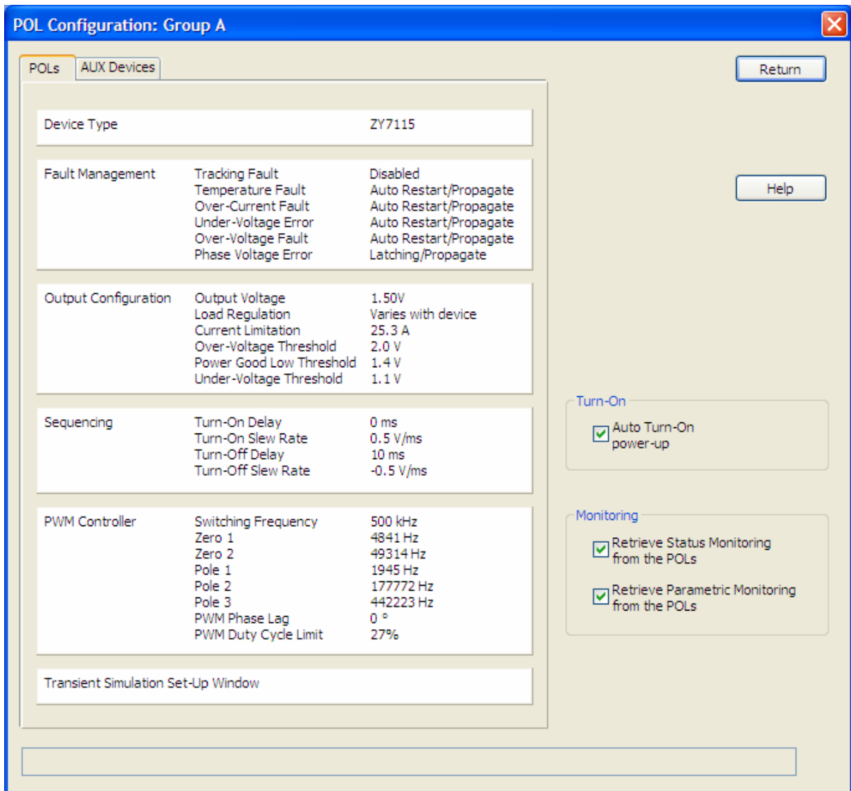
Figure 10. POL Group Configuration Window
