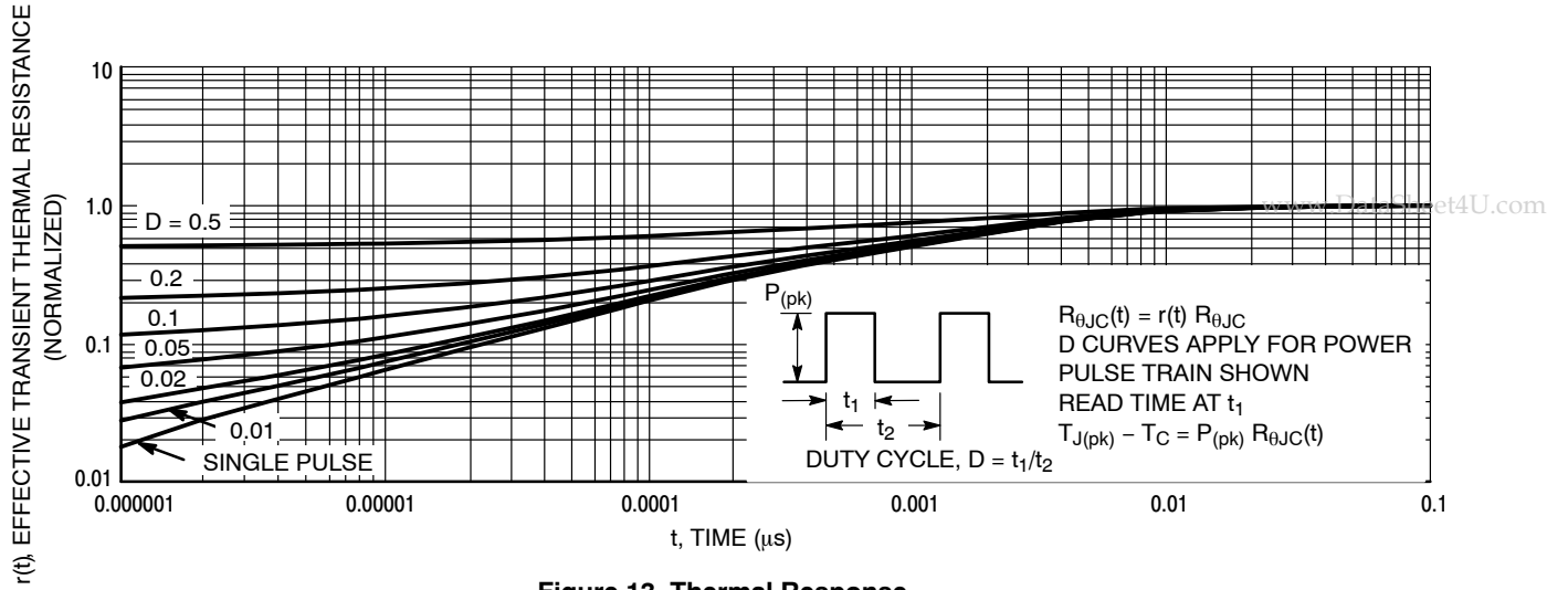
Figure 13. Thermal Response
