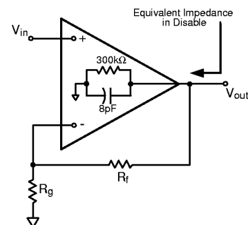
Fig. 2 Equivalent Disabled Output Impedance
