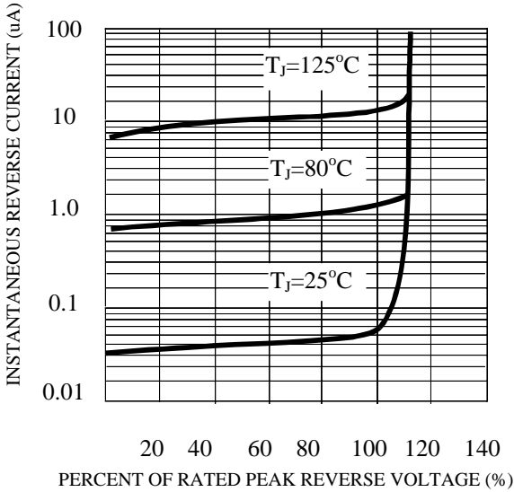
FIG. 3-TYPICAL REVERSE CHARACTERISTICS
