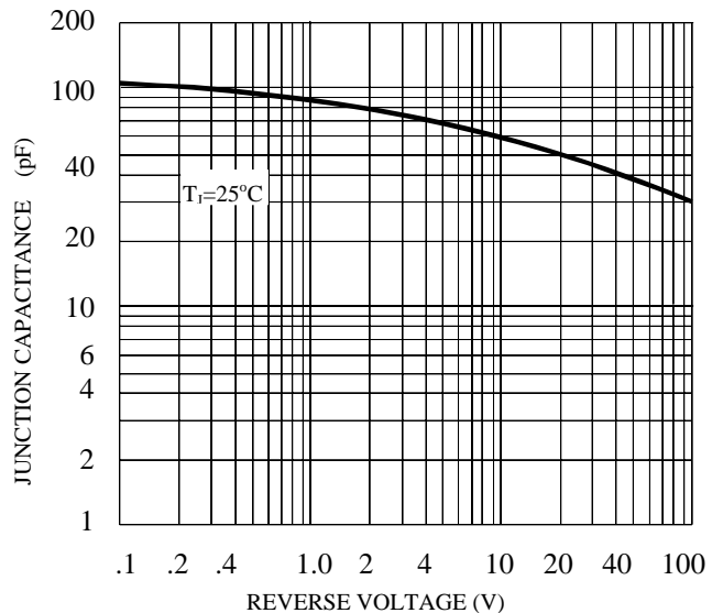
FIG. 6-TYPICAL JUNCTION CAPACITANCE
