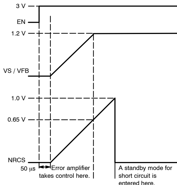
Figure 13. Powerup (NCP3520 (1.2 V) Version Shown)
