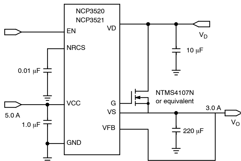
Figure 1. Application Diagram
