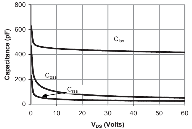
Figure 8: Capacitance Characteristics
