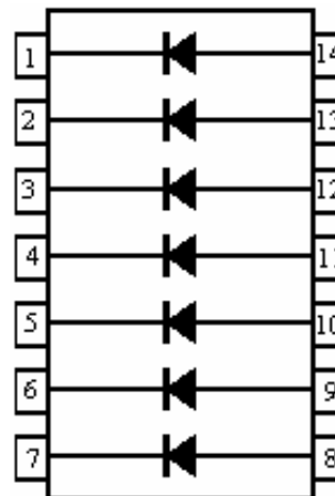
CIRCUIT CONFIGURATION
