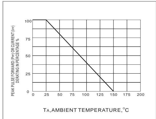
Fig.2 DERATING CURVE
