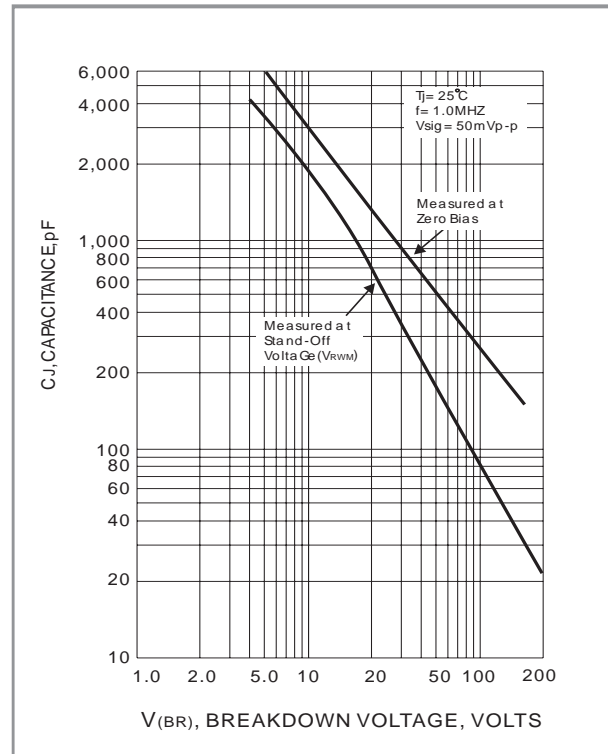
Fig.4 TYPICAL CAPACITANCE
