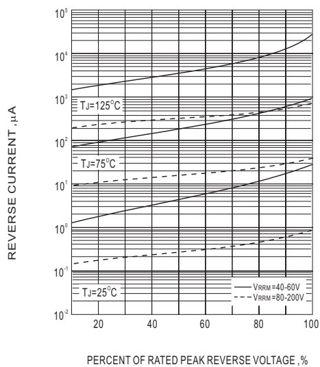
Fig.3- TYPICAL REVERSE CHARACTERISTIC
