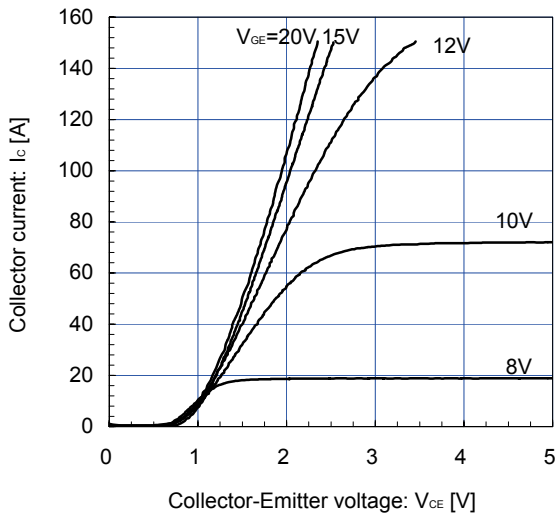
Collector current vs. Collector-Emittter voltage (typ.) T_J = 25^\circ\text{C} / \text{chip}
