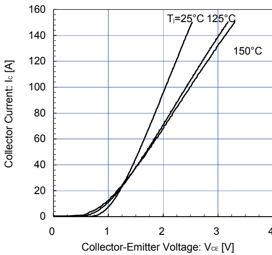
Collector current vs. Collector-Emittter voltage (typ.) V_{GE} = 15\text{V} / \text{chip}
