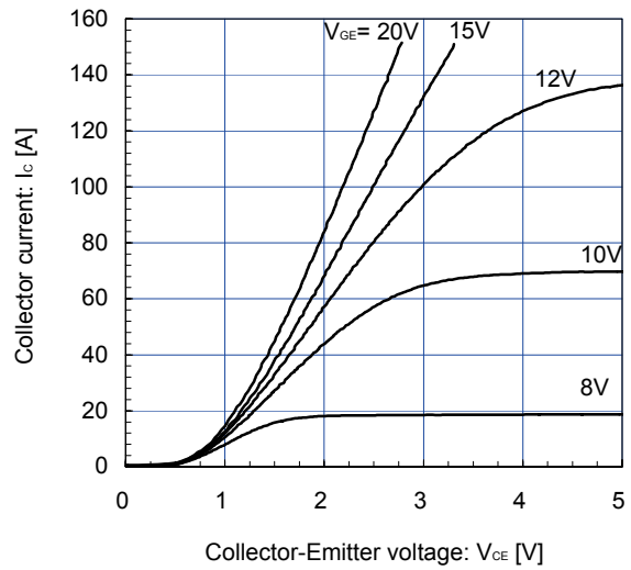
Collector current vs. Collector-Emittter voltage (typ.) T_J = 150^\circ\text{C} / \text{chip}
