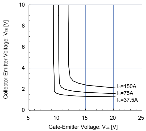
Collector-Emittter voltage vs. Gate-Emittter voltage T_J = 25^\circ\text{C} / \text{chip}
