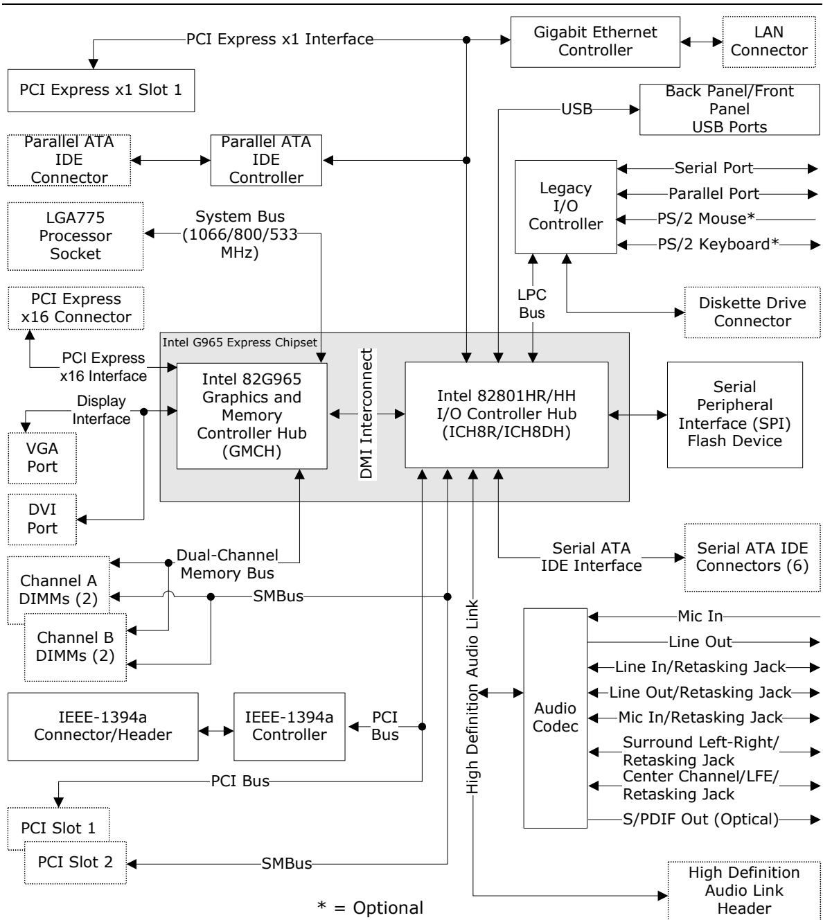
Figure 2. Block Diagram
