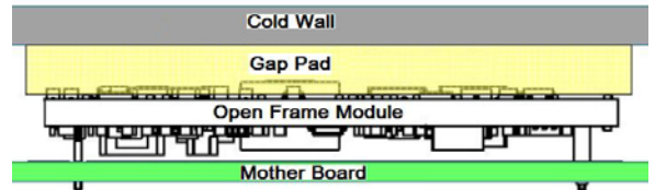
Figure 19. Cold Wall Mounting
