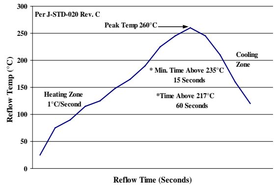
Figure 25. Recommended linear reflow profile using Sn/Ag/Cu solder.
