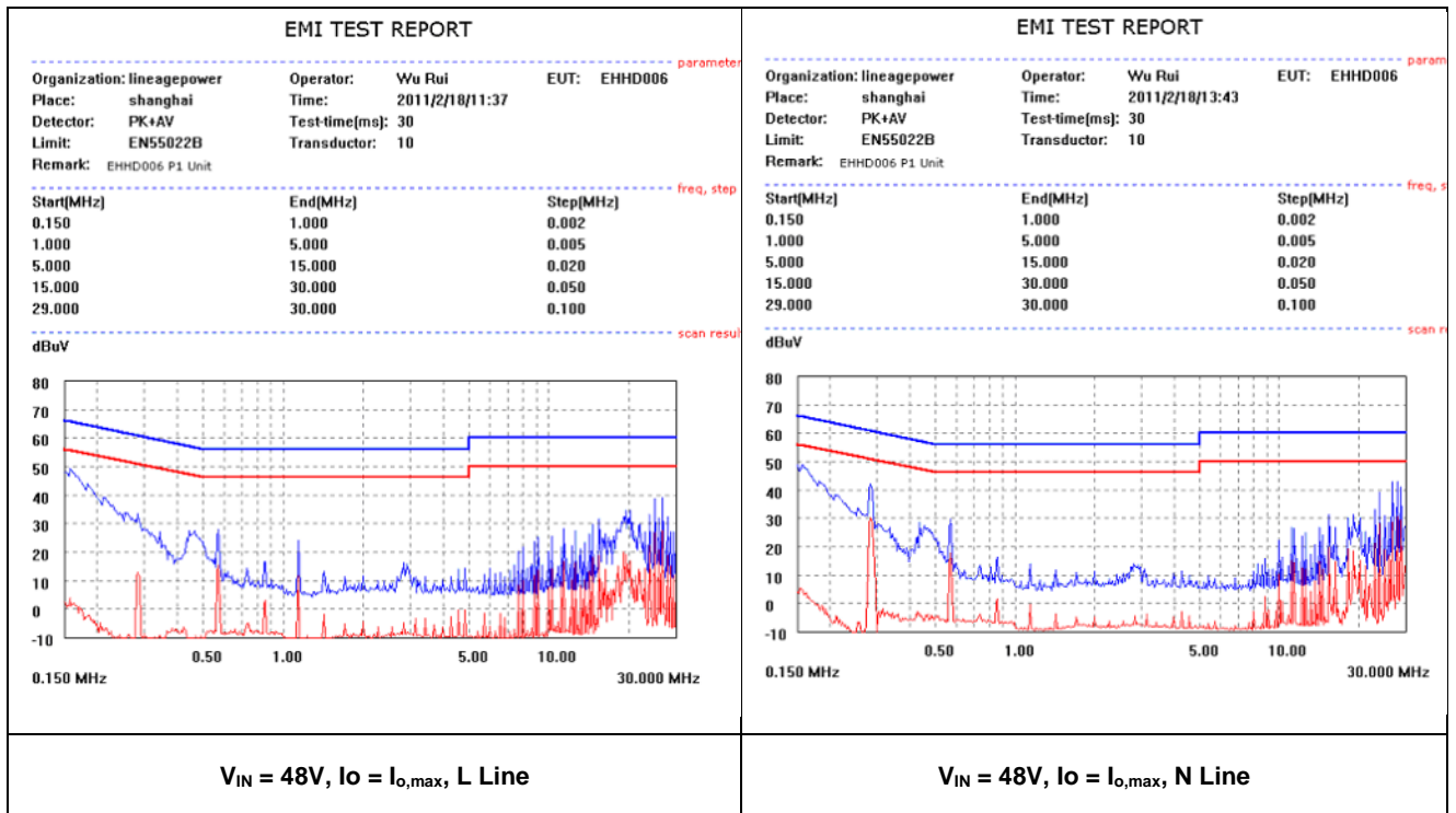
Figure 26. EMC Considerations.
