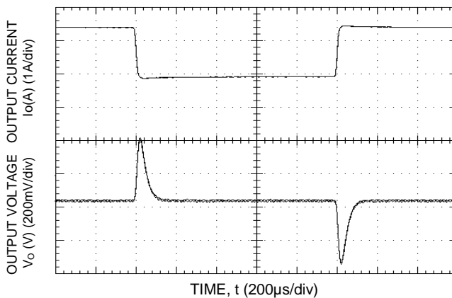
Figure 5. Transient Response to 0.1A/μS Dynamic Load Change from 50% to 75% to 50% of full load, V_{IN}=48V , C_o > 100\mu F .
