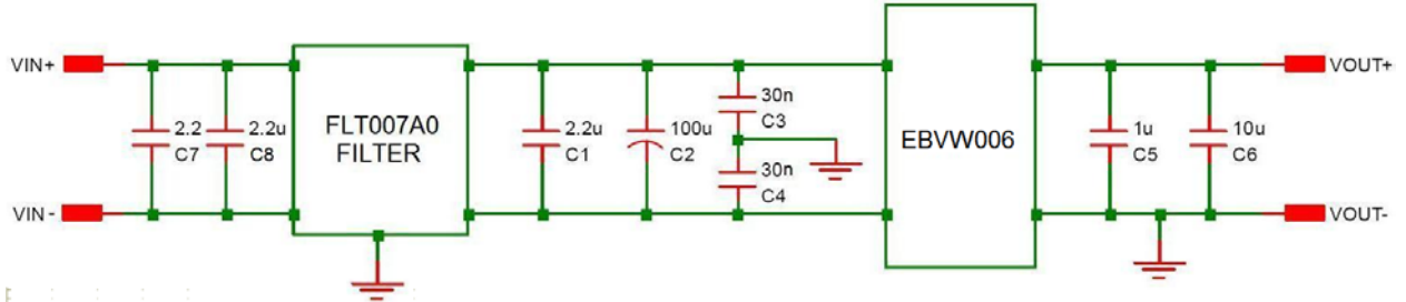
Figure 26. EMC Considerations.
