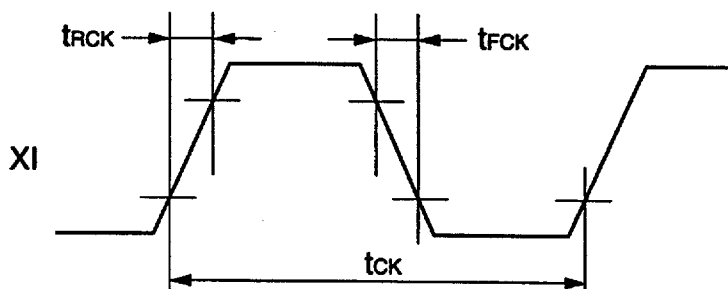
Fig.1 Master clock timing
