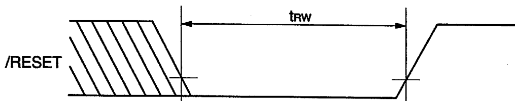
Fig.2 Reset timing
