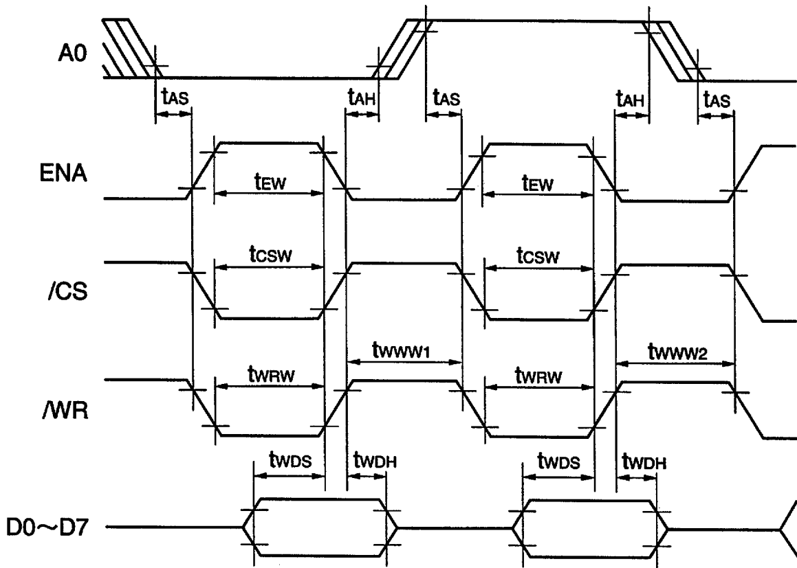
Fig.3 CPU interface timing
