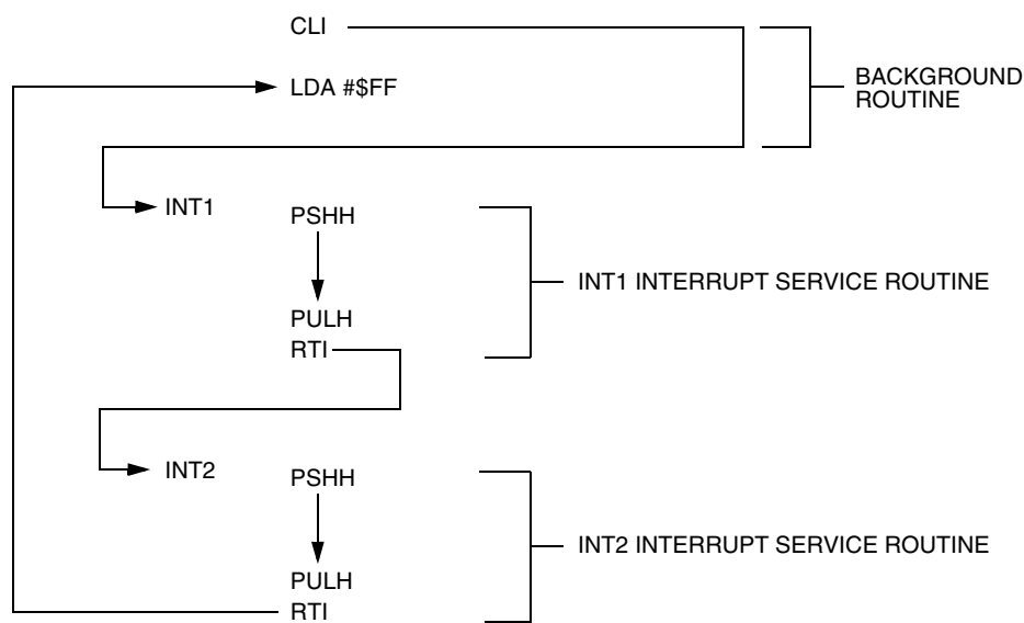
Figure 9-11. Interrupt Recognition Example
