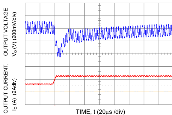
Figure 21. Transient Response to Dynamic Load Change from 50% to 100% at 28Vin, Cext - 1x10uF ceramic, CTune=150pF & RTune=220Ω
