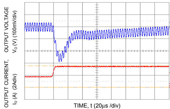
Figure 15. Transient Response to Dynamic Load Change from 50% to 100% at 28Vin, C ext - 3x10uF ceramic, C Tune =470pF & R Tune =150Ω
