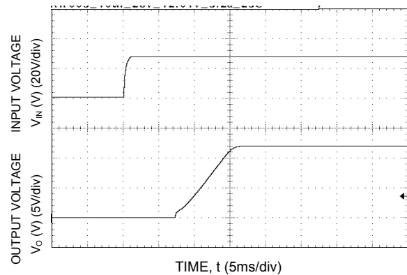
Figure 17. Typical Start-up Using Input Voltage ( V_{IN} = 28V , I_o = I_{o,max} ).
