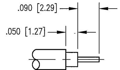
CABLE TRIMMING DIMENSIONS
