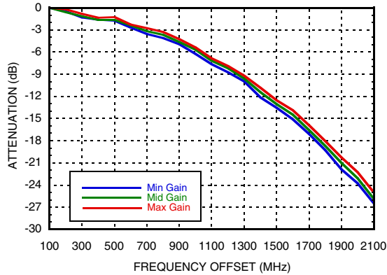
Figure 19. Single Sided Passband Response vs. IF Gain [5][6]
