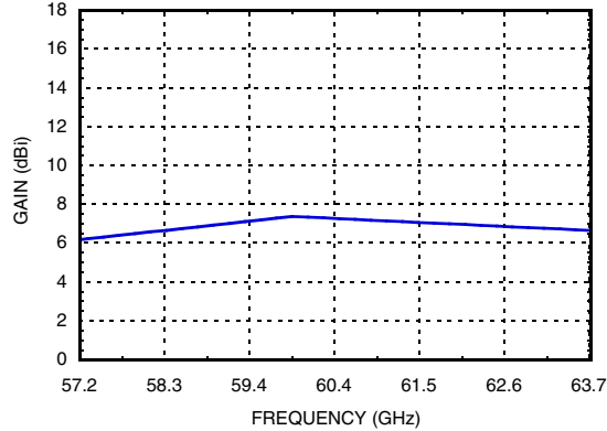
Figure 1. Antenna Peak Gain vs. Frequency [1]
