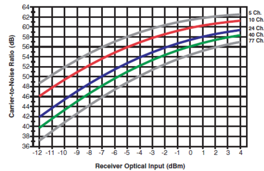
Carrier-to-Noise Performance
