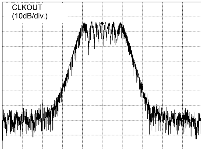
Figure 27. CLKOUT±0.75% Modulation Spectrum
