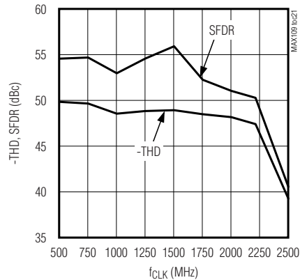
-THD, SFDR vs. CLOCK SPEED ( f_{IN} = 1600MHz , A_{IN} = -1dBFS )
