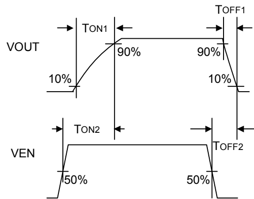
Fig.2 Timing diagram
