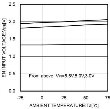
Fig.6 EN threshold voltage (Low level input voltage)
