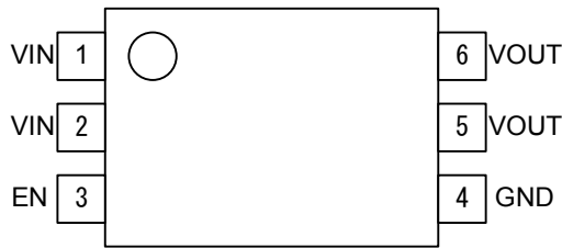
Fig.28 Pin configuration
