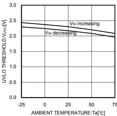
Fig.12 UVLO threshold voltage
