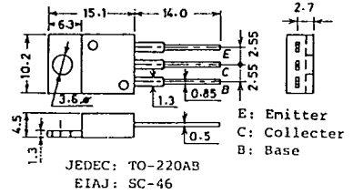
Case Outline—[2012]
