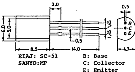
Case Outline—[2006A]
