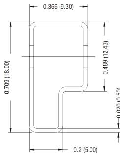
4 PIN SIP Tube
