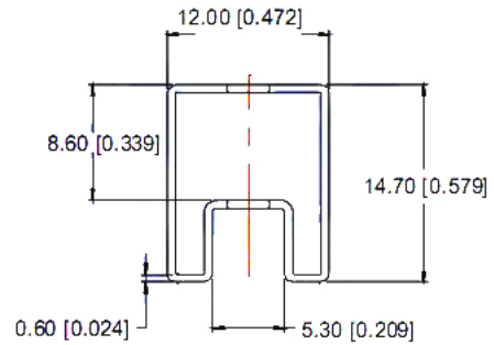
14 PIN DIP Tube
