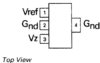
SOT89 Package Suffix - Z
