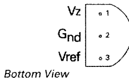
TO92 Package Suffix - C
