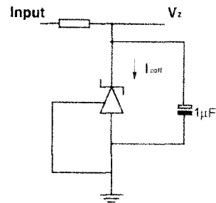
Fig 3 – Test Circuit for Off State current
