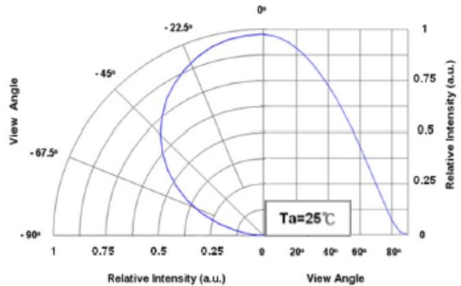
Radiation Pattern
