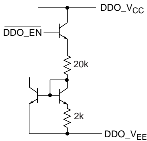
Fig. 14 \overline{DDO\_EN} Circuit
