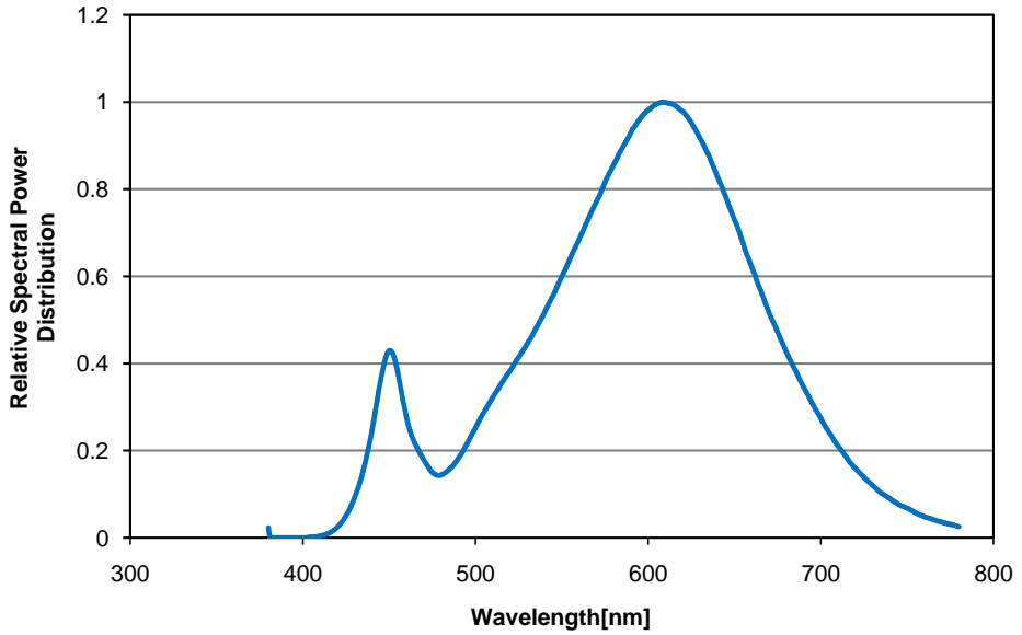
Warm White Relative Spectral Distribution vs. Wavelength Characteristic
