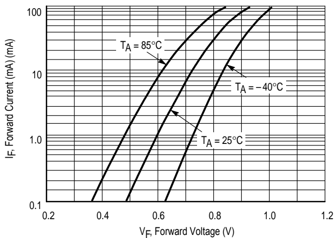
Figure 2. Forward Voltage
