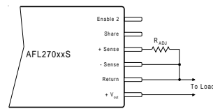
Figure V. Connection for V_{OUT} Adjustment
