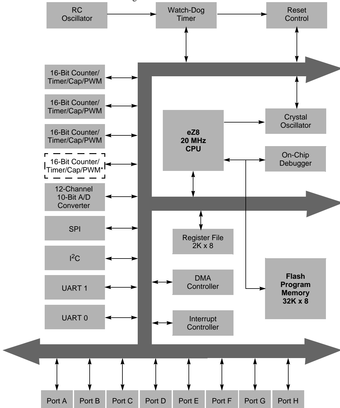
Figure 1. Z8F320x Block Diagram
