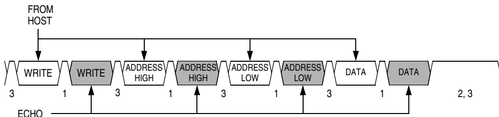
Figure 18-10. Read Transaction
