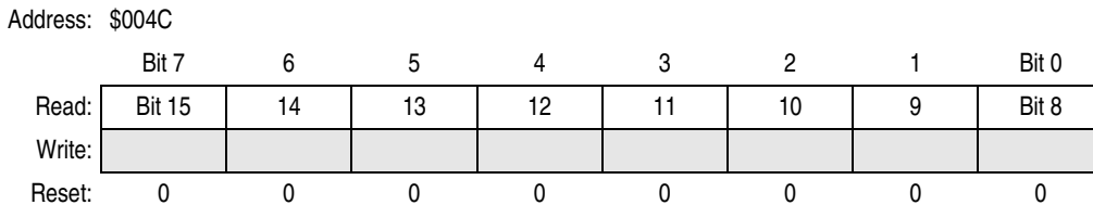
Figure 12-3. PIT Counter Registers (PCNTH–PCNTL)
