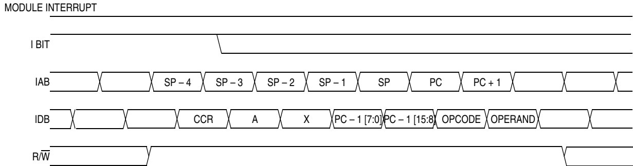
Figure 15-10. Interrupt Recovery
