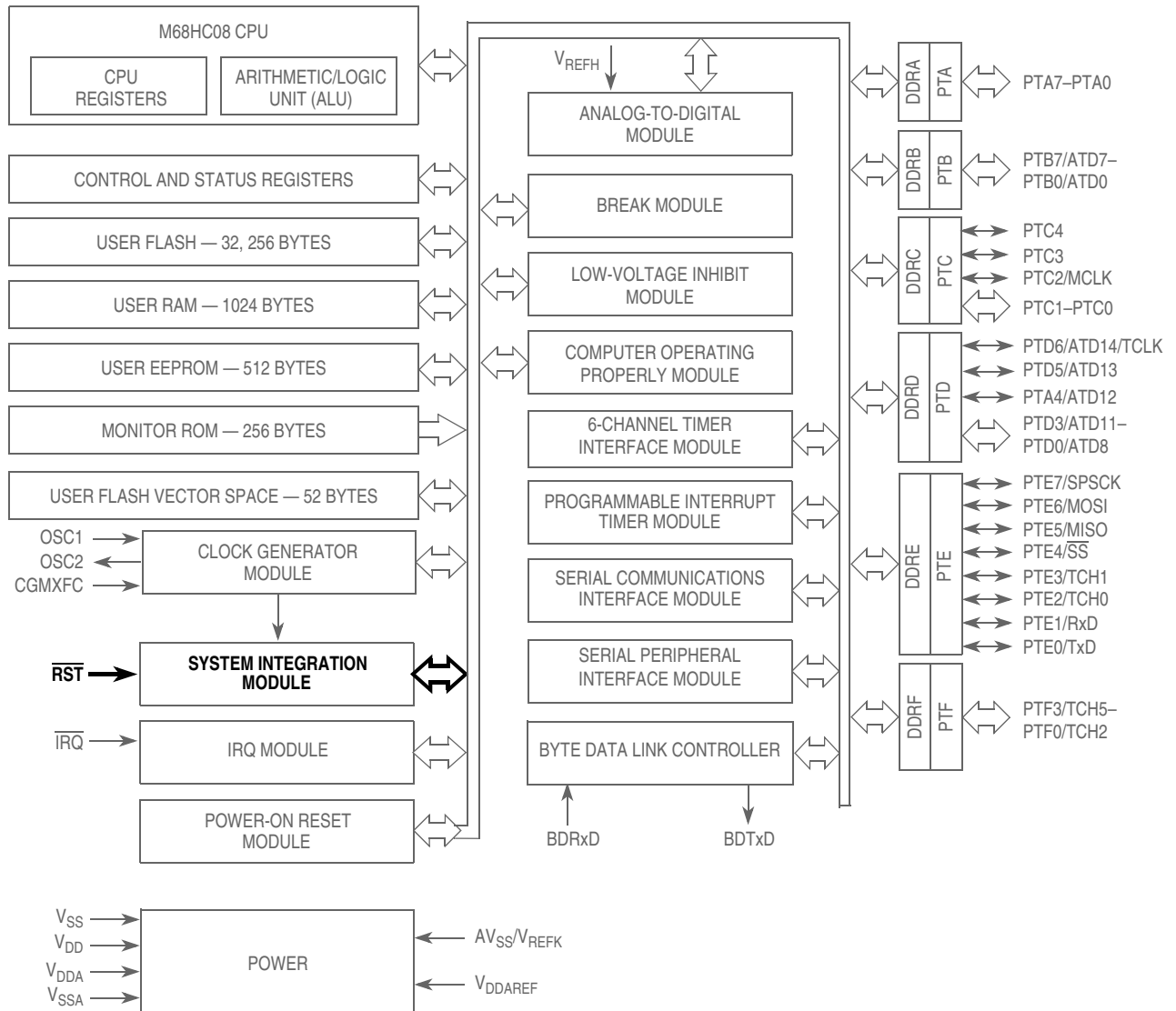
Figure 15-1. Block Diagram Highlighting SIM Block and Pins
