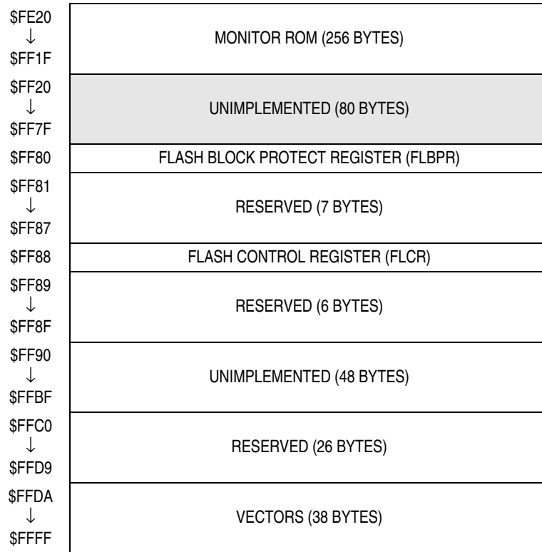
Figure 2-1. Memory Map (Continued)
