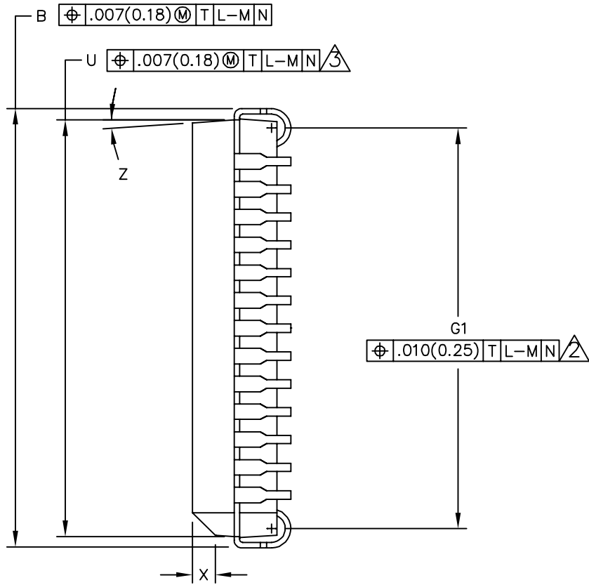
VIEW D-D
