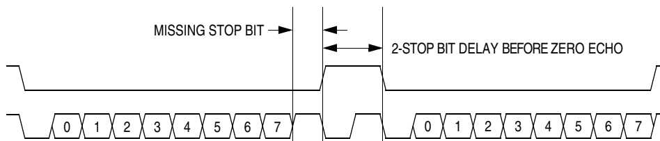
Figure 18-9. Break Transaction
