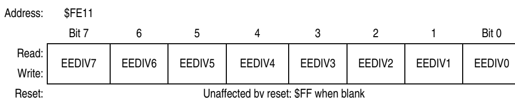
Figure 2-10. EEPROM Divider Nonvolatile Register Low (EEDIVLNVR)
