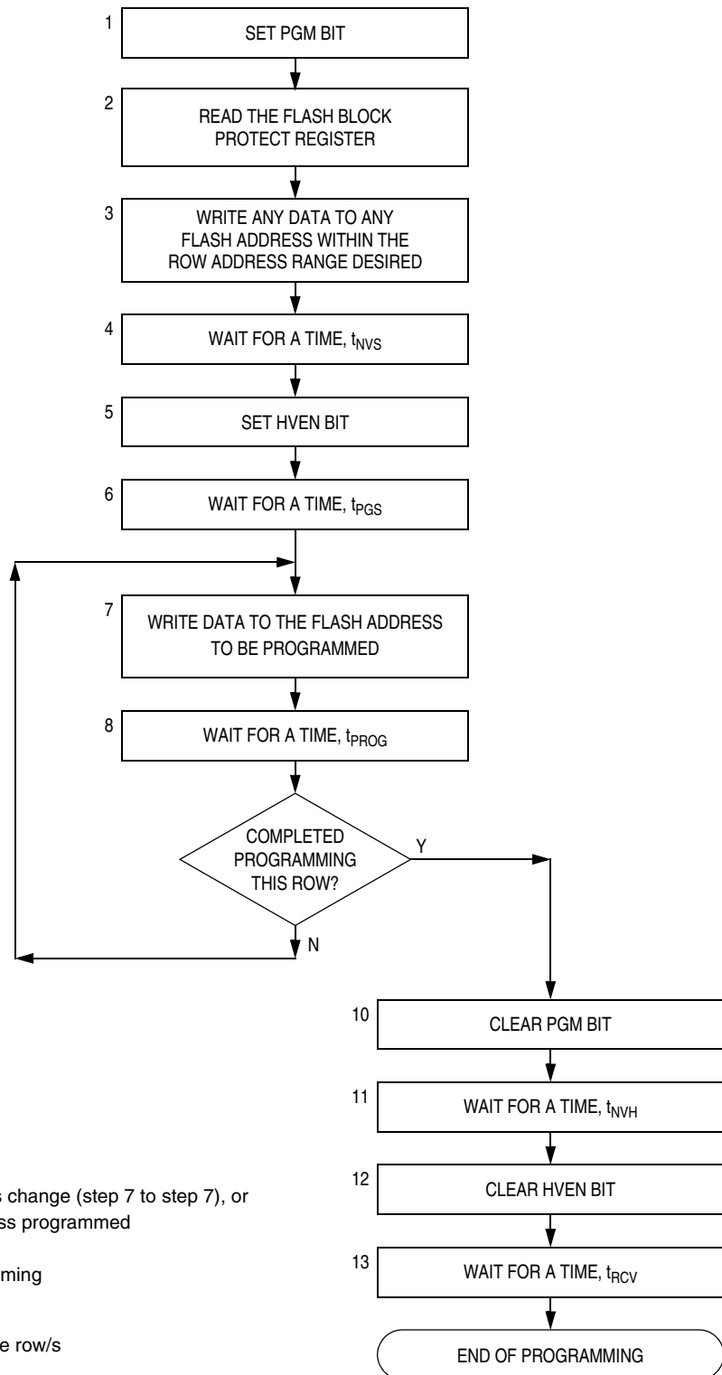
Figure 2-14. FLASH Programming Algorithm Flowchart
