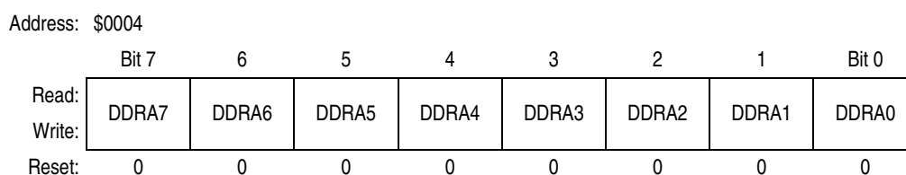
Figure 13-2. Data Direction Register A (DDRA)
