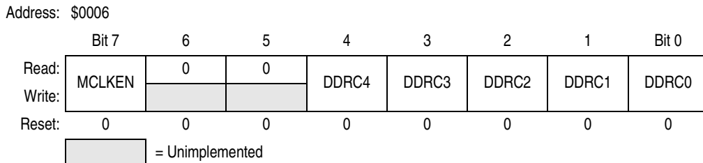
Figure 13-8. Data Direction Register C (DDRC)
