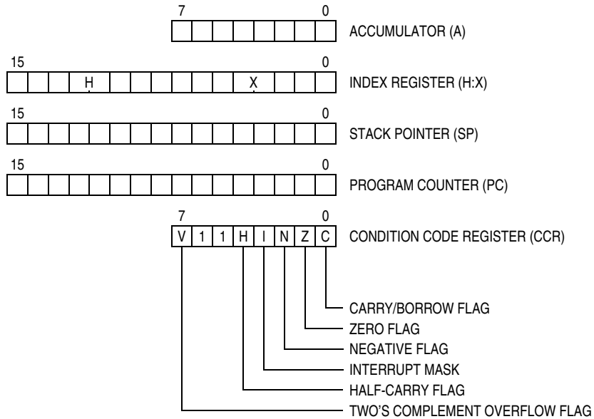
Figure 9-1. CPU Registers
