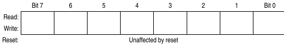
Figure 9-2. Accumulator (A)
