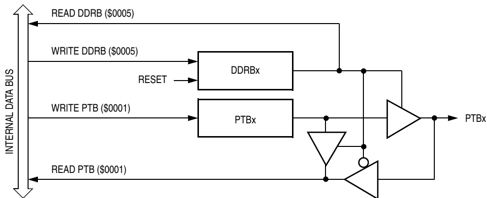
Figure 13-6. Port B I/O Circuit
