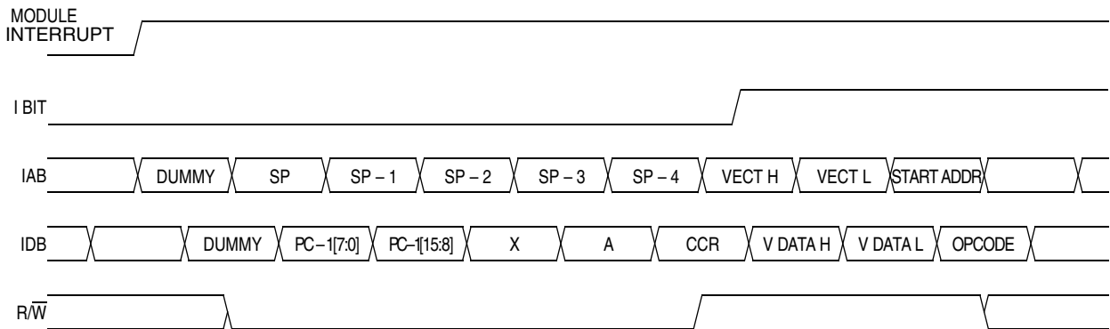
Figure 15-8. Interrupt Entry
