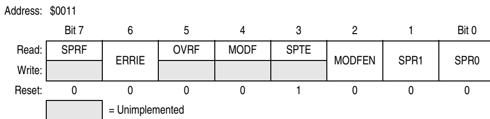
Figure 16-13. SPI Status and Control Register (SPSCR)
