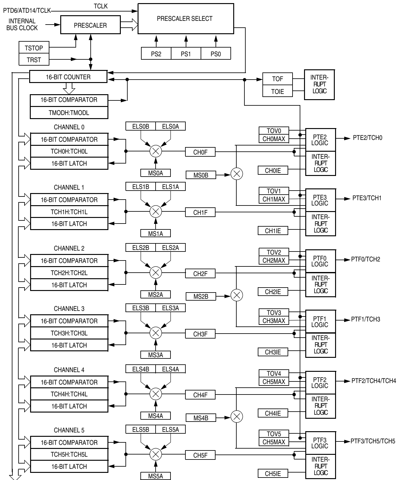
Figure 17-2. TIM Block Diagram
