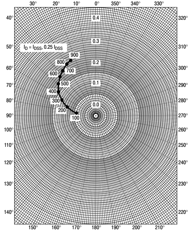
Figure 6. S_{12s}
