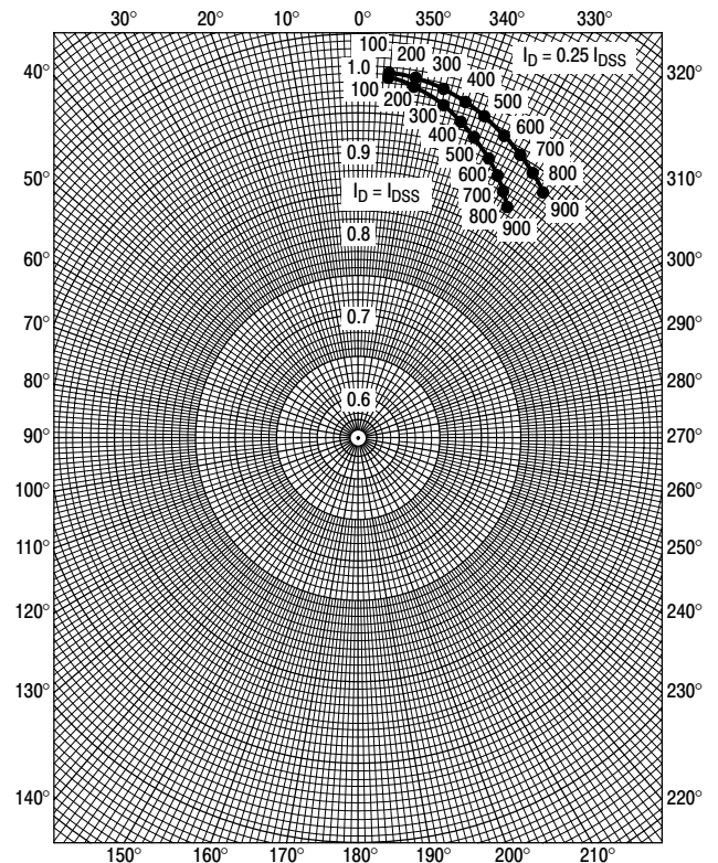
Figure 8. S_{22s}
