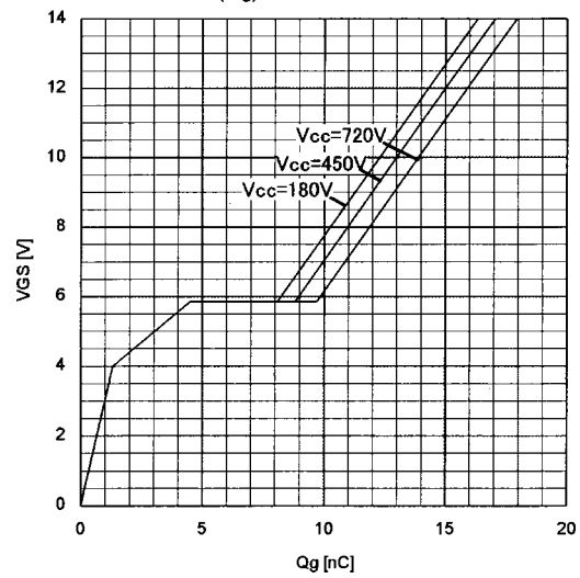
Typical Gate Charge Characteristics V_{GS}=f(Q_g):I_D=2.6A,T_{ch}=25\text{ }^\circ C
