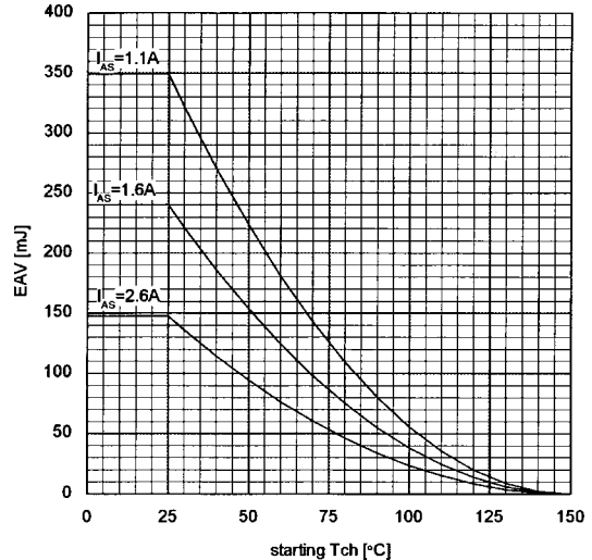
Maximum Avalanche Energy vs. starting Tch E_{(AV)}=f(\text{starting } T_{ch}):V_{cc}=100V,I_{(AV)}\le 2.6A
