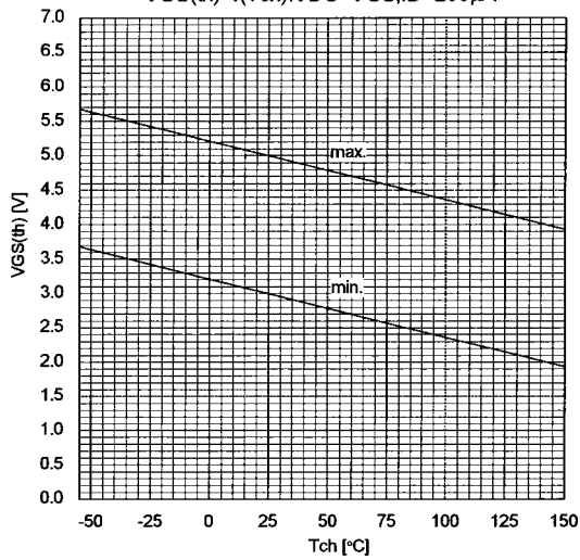
Gate Threshold Voltage vs. Tch V_{GS(th)}=f(T_{ch}):V_{DS}=V_{GS},I_D=250\mu A
