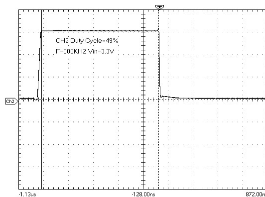
Channel 2 Duty Cycle @ VCC= 3.3V, C1= 15pF
