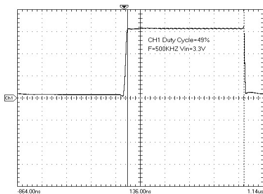
Channel 1 Duty Cycle @ VCC= 3.3V, C1= 15pF
