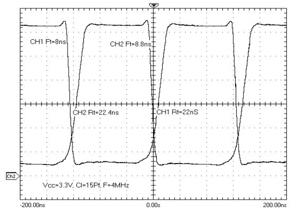
Waveform @ 4MHz and VCC= 3.3V (vertical scale 500mV/div)
