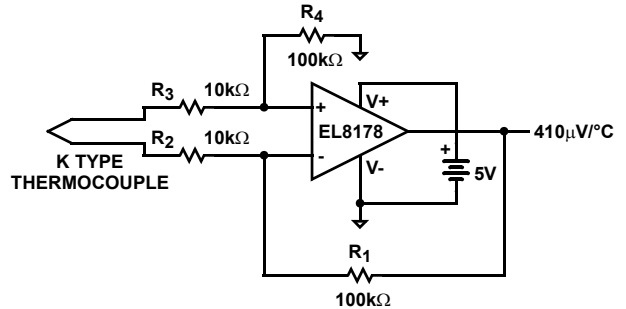
FIGURE 30. THERMOCOUPLE AMPLIFIER
