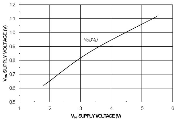
Figure 9. V ON Low Voltage vs. Input Voltage
