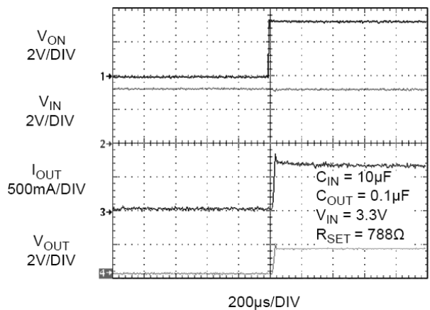
Figure 22. Current Limit Response Time (Output is Loaded by 2.2Ω, C OUT =0.1µF)
