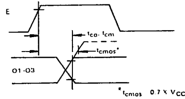
FIGURE 7 - OUTPUT DELAY
