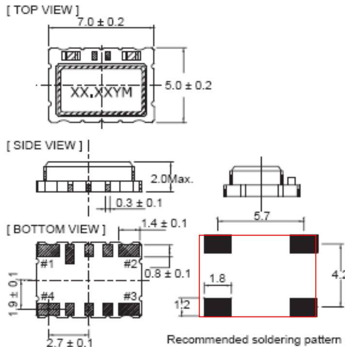
Figure 3, Package drawing
