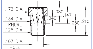
8016-0-15-XX-07-XX-10-0 Press-fit in .131 mounting hole
