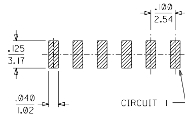
RECOMMENDED PCB LAYOUT: COMPONENT SIDE
