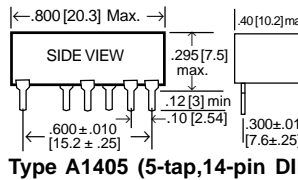
Type A1405 (5-tap, 14-pin DIP)
