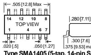
Type SMA1405 (5-tap, 14-pin SO)
