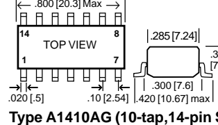
Type A1410AG (10-tap, 14-pin SM)
