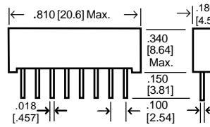
Type SA0805 (5-tap, 8-pin SIP)
