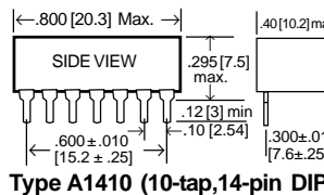
Type A1410 (10-tap, 14-pin DIP)
